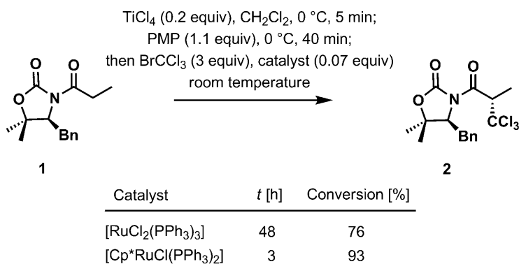
Scheme 4. Comparison between [\text{RuCl}_2(\text{PPh}_3)_3] and [\text{Cp}^*\text{RuCl}(\text{PPh}_3)_2] as the redox catalyst for radical generation. \text{Cp}^* = 1,2,3,4,5 -pentamethylcyclopentadienyl anion.
